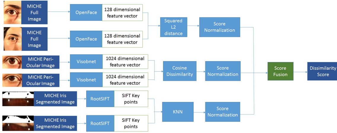
Fig. 1: Schematic representation of proposed model 1.
