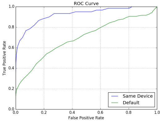
Fig. 2: OpenFace ROC
