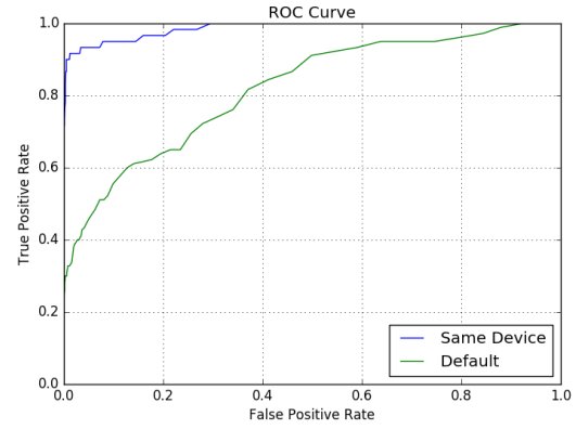
Fig. 5: Model 2 ROC
