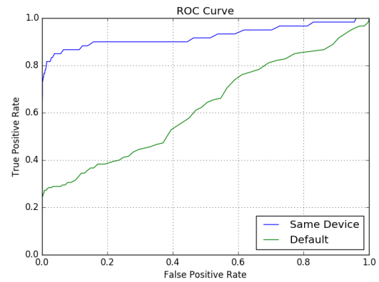
Fig. 7: Visobnet ROC
