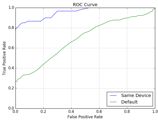
Fig. 4: Model 1 LR ROC
