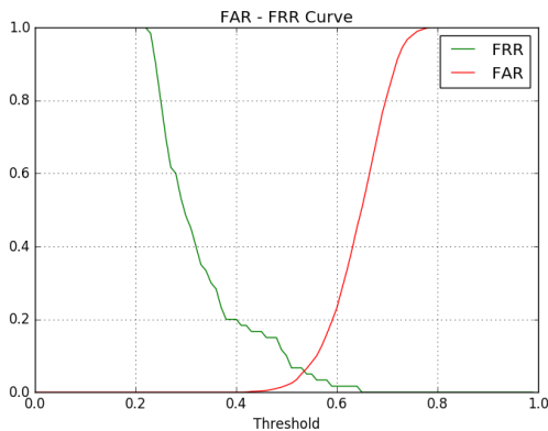
Fig. 9: Hybrid Model FAR-FRR in the SD_SE paradigm
