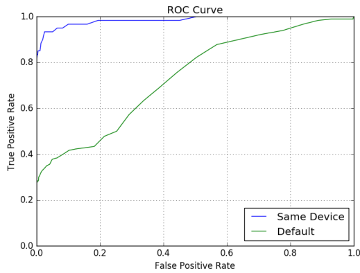
Fig. 8: Hybrid Model ROC
