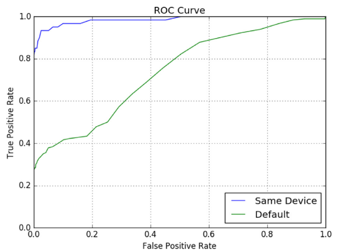
Fig. 10. Hybrid model receiver operating characteristics on MICHE-II.
