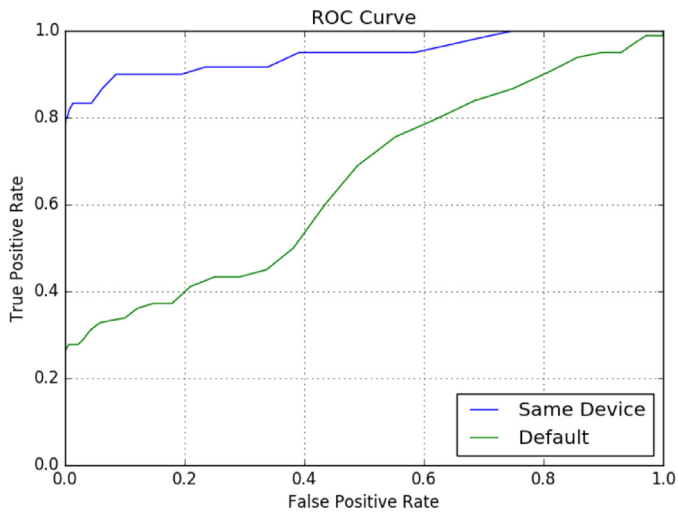
Fig. 5. Model 1 EQ ROC on MICHE-II.
