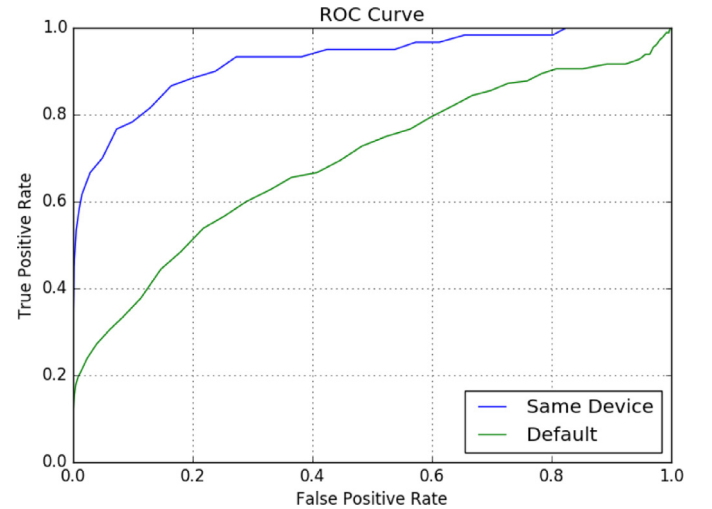
Fig. 4. OpenFace ROC on MICHE-II.
