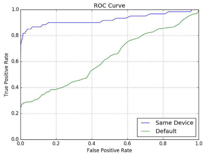
Fig. 9. VisobNet ROC on MICHE-II.
