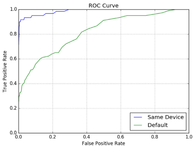
Fig. 7. Model 2 ROC on MICHE-II.
