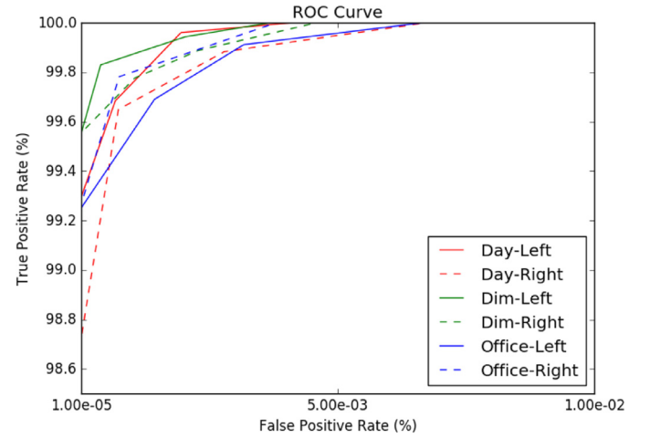
Fig. 15. ROC for I-Phone on VISOB.
