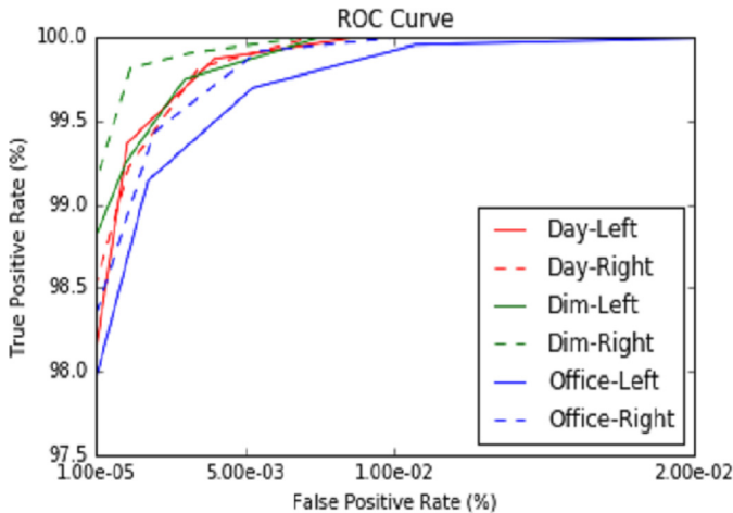
Fig. 13. ROC for Samsung on VISOB.
