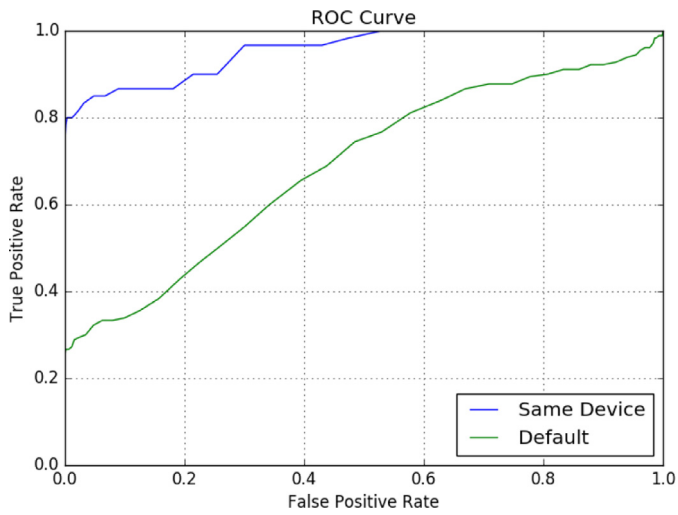
Fig. 6. Model 1 LR ROC on MICHE-II.
