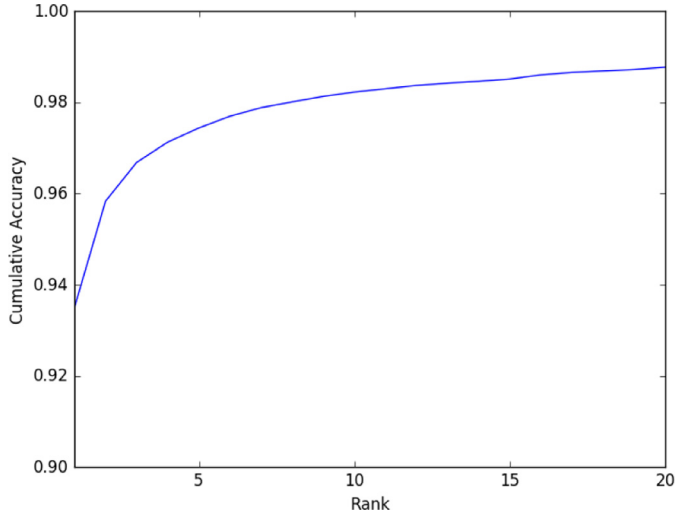
Fig. 12. Cumulative match curve for VISOB database.
