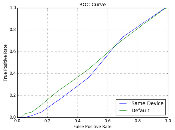
Fig. 8. Root SIFT ROC on MICHE-II.
