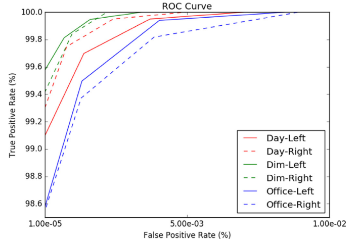
Fig. 14. ROC for Oppo on VISOB.
